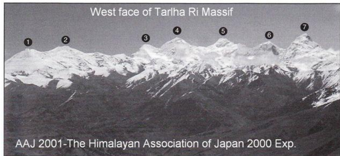
Peaks of the Tarlha Ri group, showing 1. Mt. Zhemazhenyon (6480m). 2. Peak 6578m. 3. Peak 6542m. 4. Tarlha Ri (6777m) 5. Xialala Kang (6682m). 6. Peak 6241m. 7. Peak 6410m. Y. Ота
